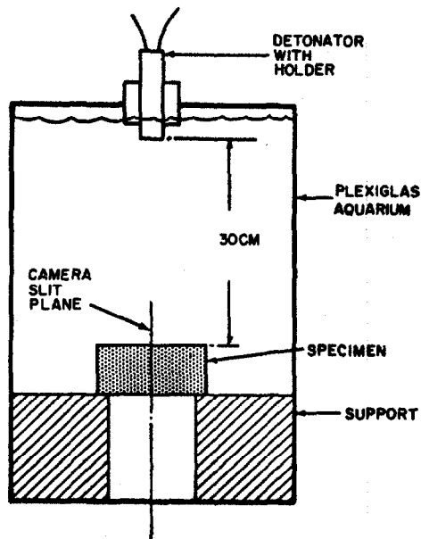
FIG 3. Arrangement for initiating and measuring weak shock waves (~100 bar)
